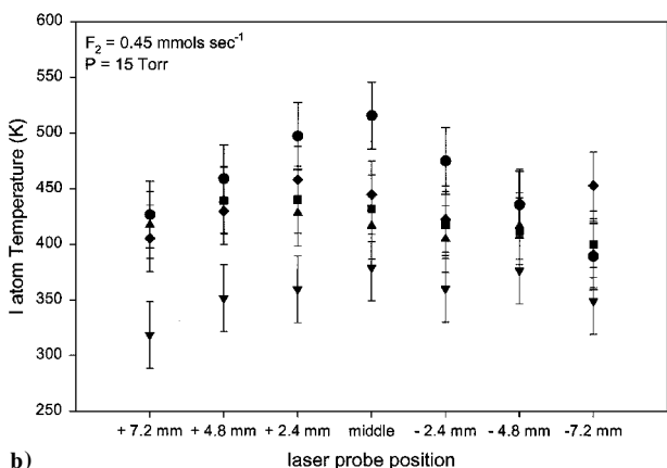
Fig. 3 Vertical profiles at various positions along the reactor; I atom laser probe can be translated along the transverse and vertical axis of the reactor. Profiles are flat for d \geq 5.5 cm.
