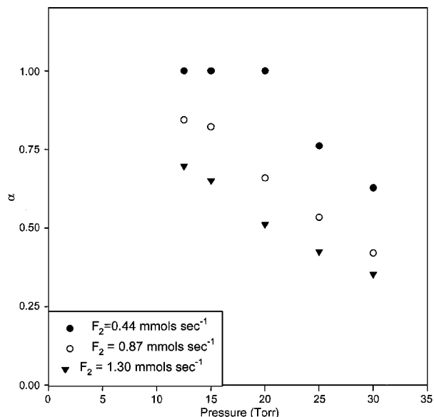
Fig. 7 Dissociation fraction vs pressure; F_2 dissociation fraction, \alpha = I_{\max}/2 \cdot F_2 , is plotted as a function of the reactor pressure.
