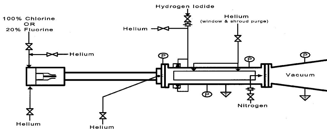
Fig. 1b Optical path for the I atom laser probe.
